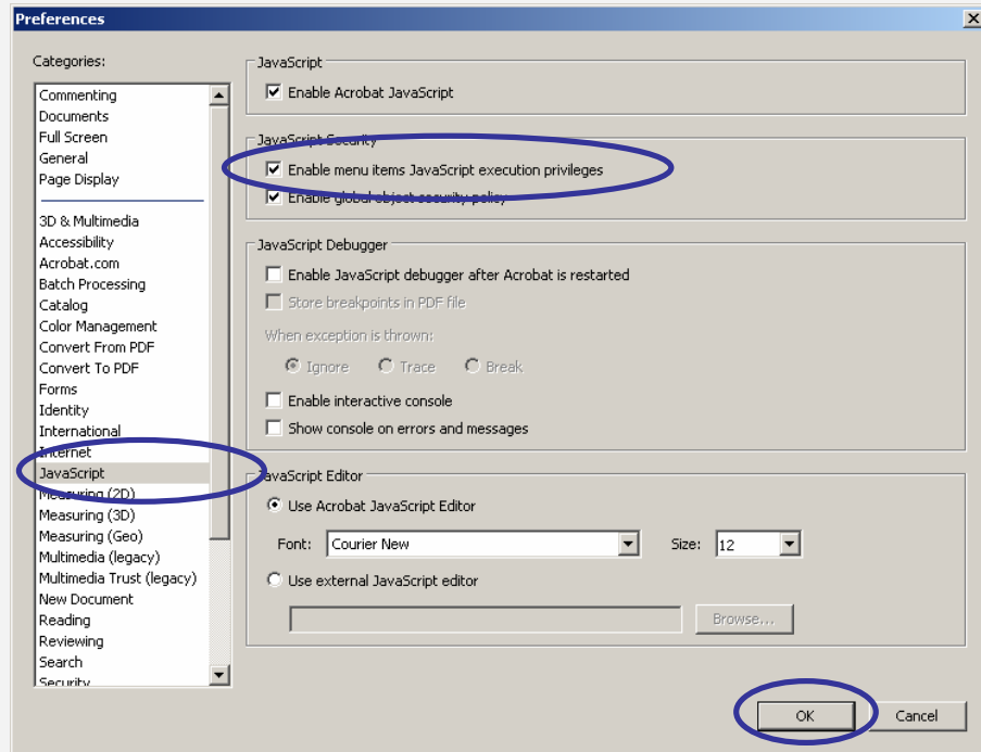
Figure 2. – Preferences dialog
