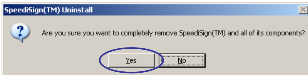
Figure 2. – Uninstall SpeediSign
